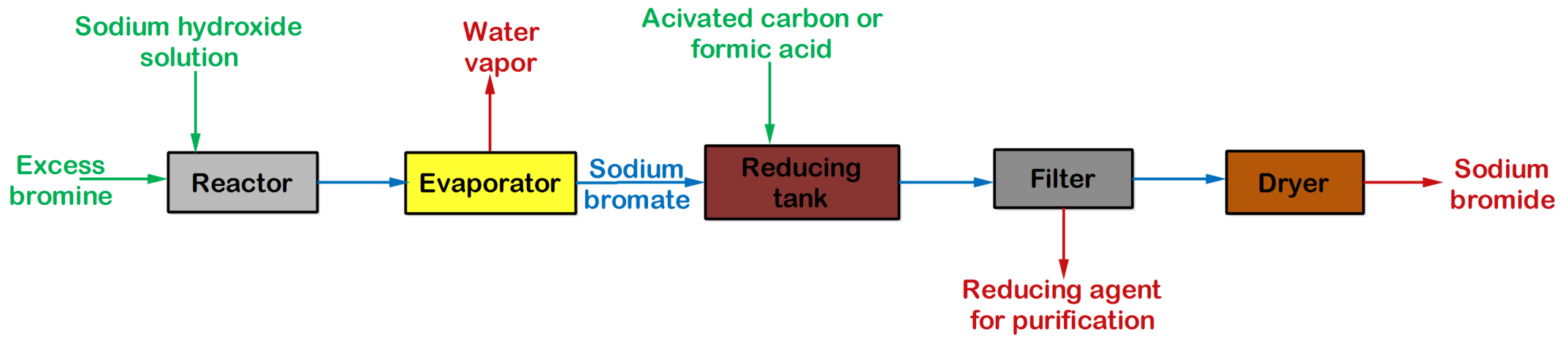
Figure: Manufacture of sodium bromide by excess bromine
